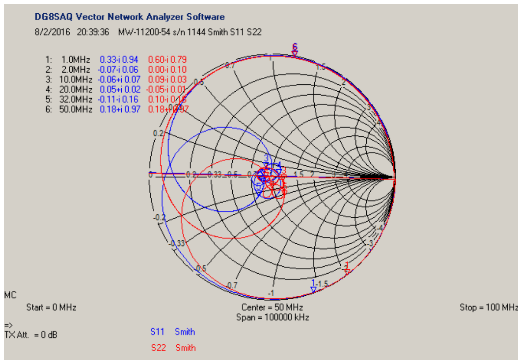
Figure 5 ~ Typical Smith Chart from the VNWA-3E analyzer. The black lines are the grid. The blue and red traces show the input (s11) and output (s22) normalized impedance over the frequency range indicated. The normalized impedance is at chart center so the traces near the center indicate a good match (low reflection coefficient) and traces along the periphery indicate a poor match. Although the grid is based on normalized impedance (inductive reactance at top, capacitive reactance at bottom) the marker table indicates reflection coefficients.
