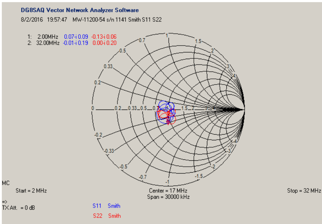
Figure 9 ~ The Smith Charts show the same information as the rectangular plots in the previous figure but only the reflection parameters S11 and S22 are shown here. Also, the frequency range has been reduced.
