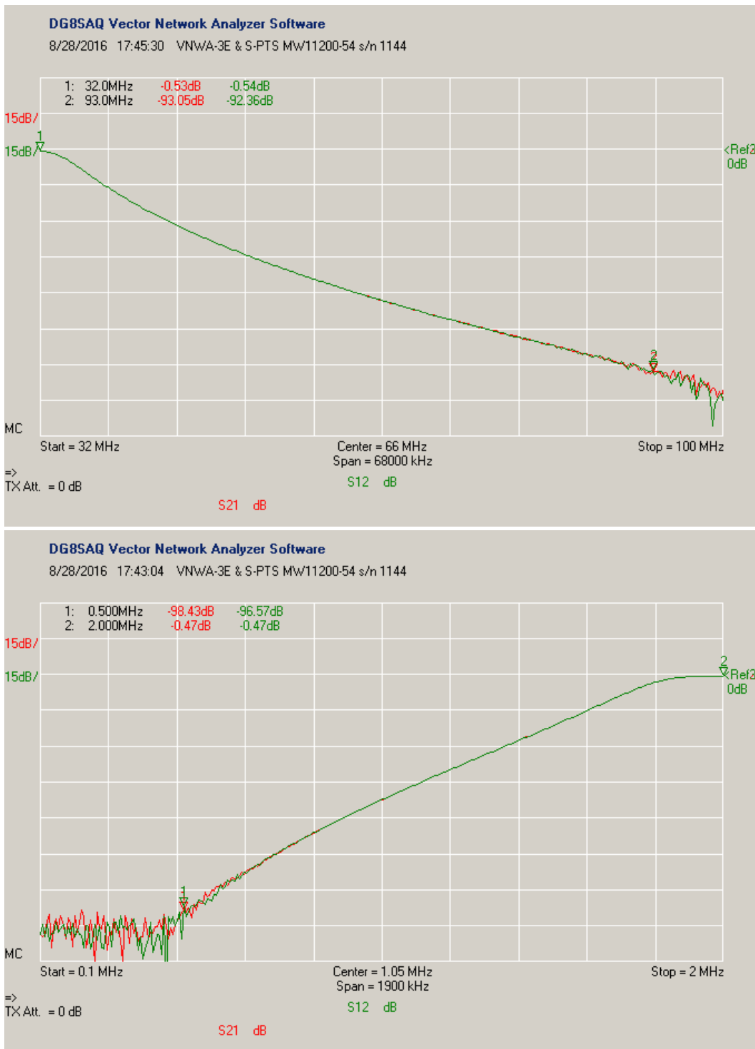
Figure 13 ~ Stopband measurements setup for 15 dB/division with 0 dB reference on the 8 th grid line. Upper : Linear frequency sweep from 32 to 100 MHz shows the loss approaches 100 dB but measurements are limited by the VNWA-3E noise floor. Lower : Linear frequency sweep from 0.1 to 2 MHz indicates the stopband loss exceeds 100 dB but, as above, the measurements are limited by the instrument's noise floor.
