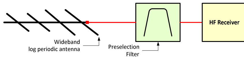
Figure 1 ~ Typical preselection filter application in which the filter is placed between the antenna and receiver to reduce out-of-band interference. Image © 2016 W. Reeve
