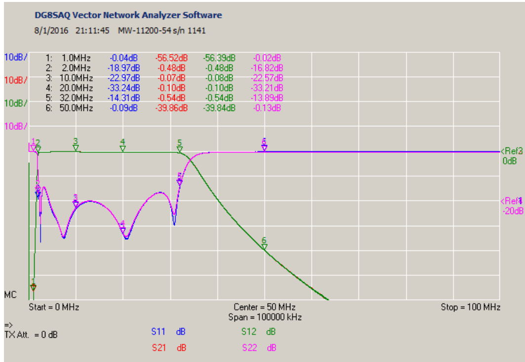
Figure 4 ~ Typical s-parameter plots from the VNWA-3E analyzer. The vertical scale shows dB. The 6 th division is the 0 dB reference. The horizontal scale is frequency from 0 to 100 MHz. The s-parameters and their corresponding trace colors are indicated at the bottom. The marker table at the upper-left shows the marker frequency and corresponding values for each trace. This plot has four traces but two are hidden underneath another trace.
