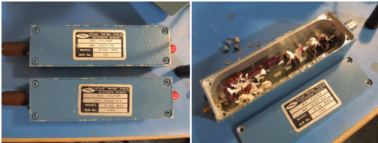
Figure 7 ~ Left : Two obviously used AEL MW-11200-54 bandpass filters. Filter dimensions are 120 x 35 x 28 mm. Right : Interior view of the filter. Typical of AEL lumped element filters, parts are soldered to pads on a simple PCB and white rubbery adhesive is used to reduce microphonics and vibration effects. These high frequency filters use toroidal inductors but AEL filters for higher frequencies use single-layer air core coils. Images © 2016 W. Reeve
