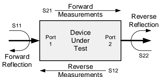
Figure 3 ~ Block diagram showing incident, reflection and transmission directions. For example, S11 is the ratio of incident voltage to reflected voltage on port 1 when port 2 is terminated in its characteristic impedance. Image © 2013 W. Reeve
