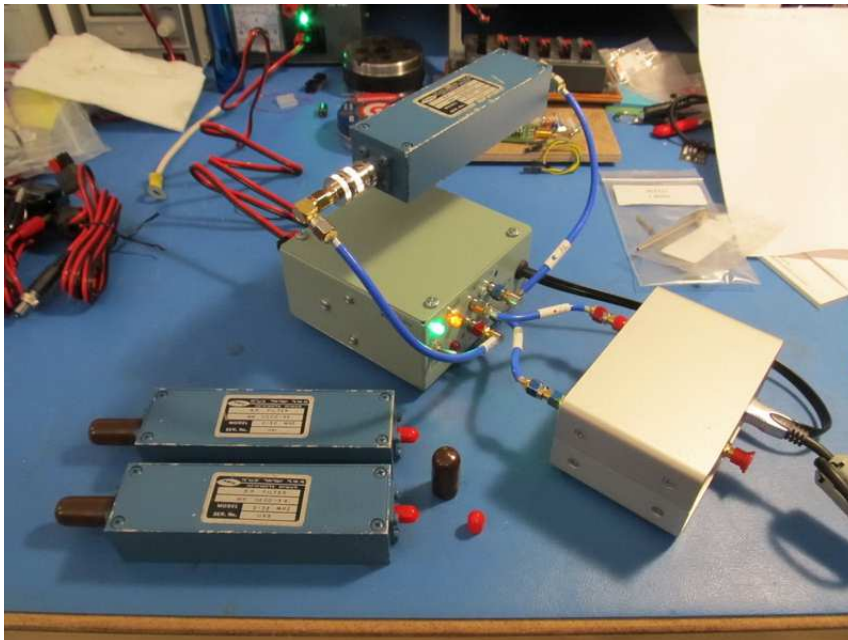
Figure 2 ~ Vector network analyzer hardware. The VNWA-3E is the silver box in the lower-right corner and the S-parameter test set is the sage green box to its left. One filter (blue box) is connected and suspended above the S-parameter test set and two additional filters are shown to the lower-left. Not shown is the PC that controls and powers the VNWA-3E through its USB port. The S-Parameter Test Set is powered by a separate 28 Vdc power supply. Image © 2016 W. Reeve
