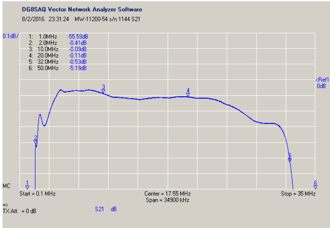
Figure 12 ~ Magnified vertical scale (0.1 dB/division) shows the passband ripple is a few tenths of a dB from 2 to 32 MHz. Although the trace is not visible at the frequencies of marker 1 and 6, valid measurements are still shown in the marker table if the measurement sweep covered the frequencies involved. Therefore, Marker 1 is valid and Marker 6 is not.
